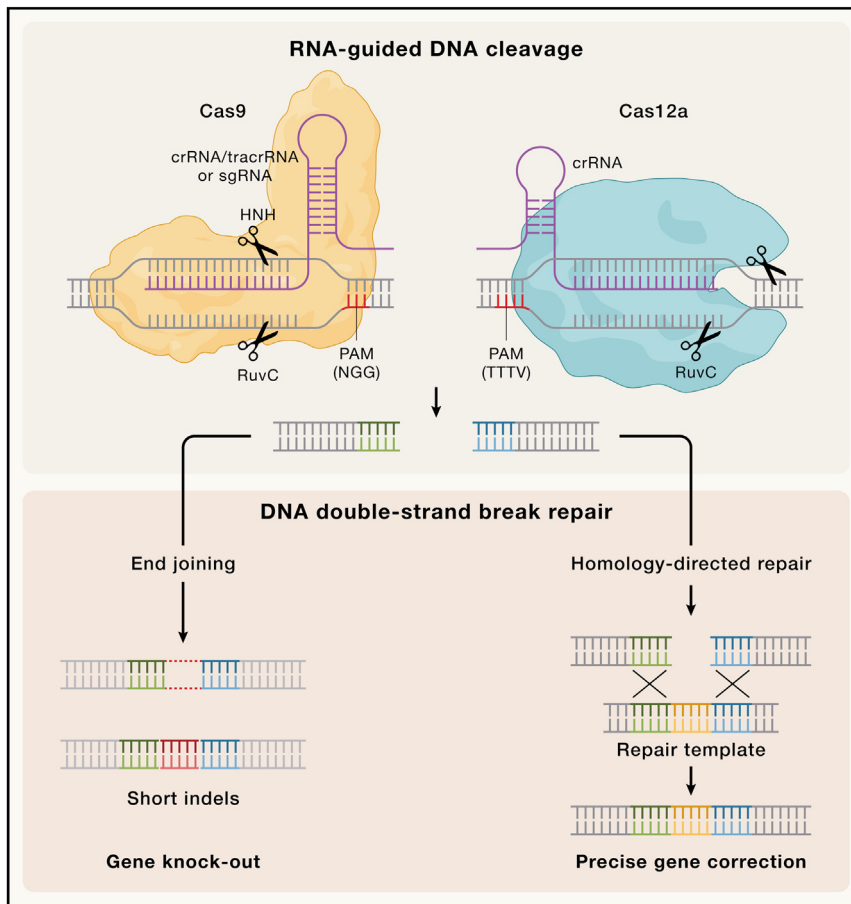
Figure 1. Molecular principles of CRISPR genome editing
