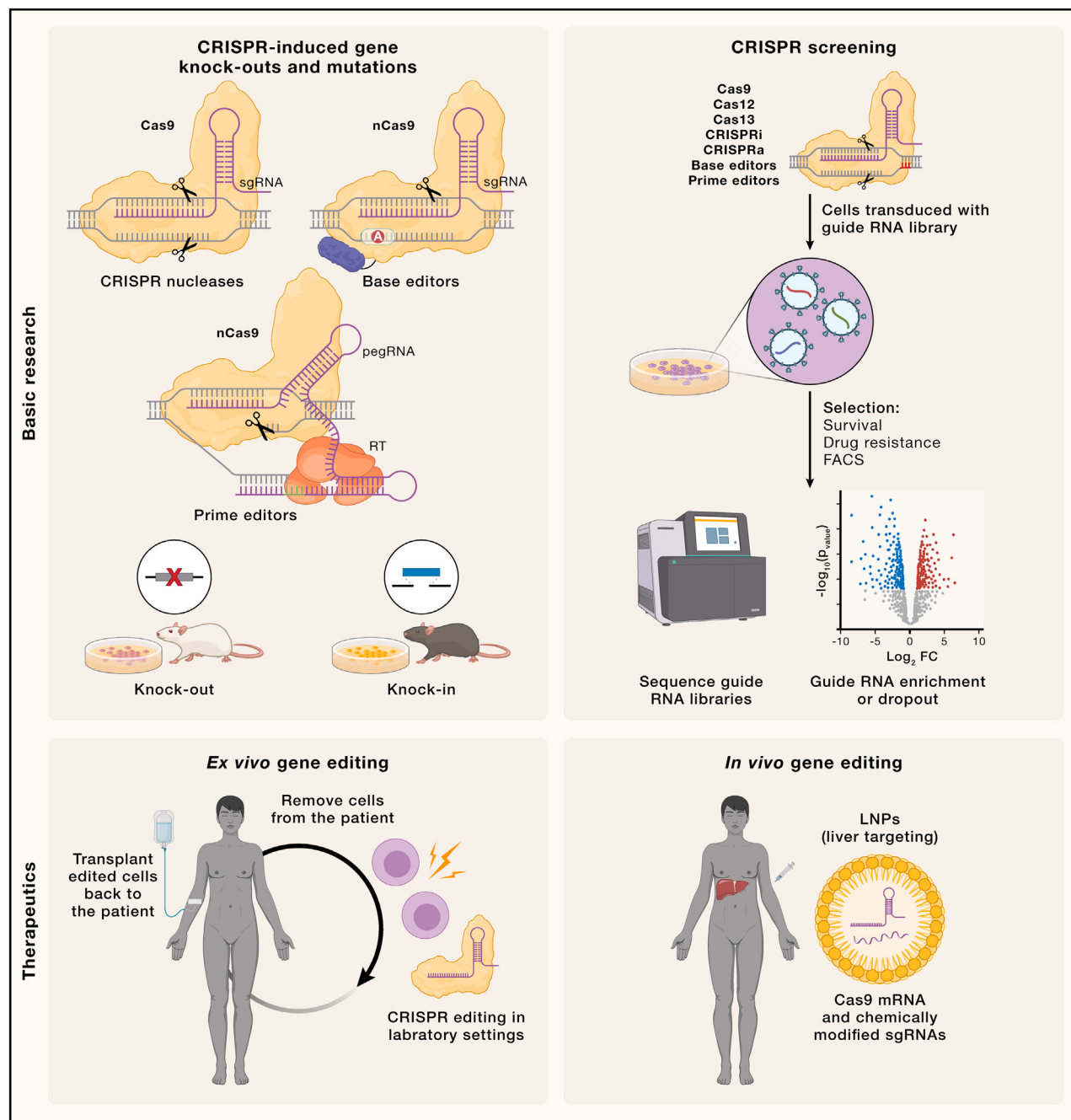
Figure 4. Applications of CRISPR genome editors relevant to human health
